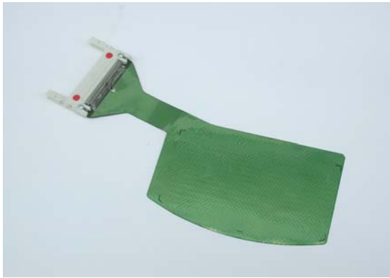
An Industrial TactArray Sensor (Brake-Pad Application)
