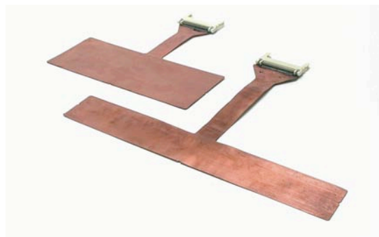
An Industrial TactArray Sensor (Brake-Pad Application)
